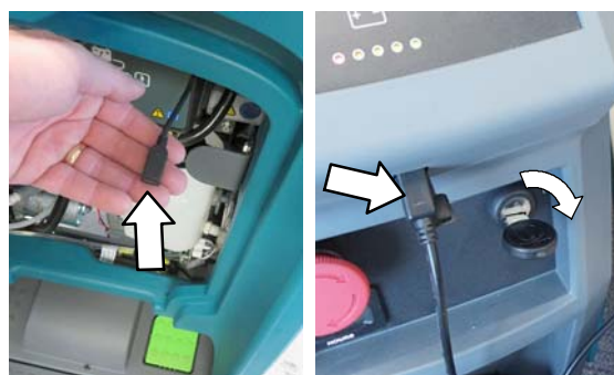
Stand-On Scrubber
