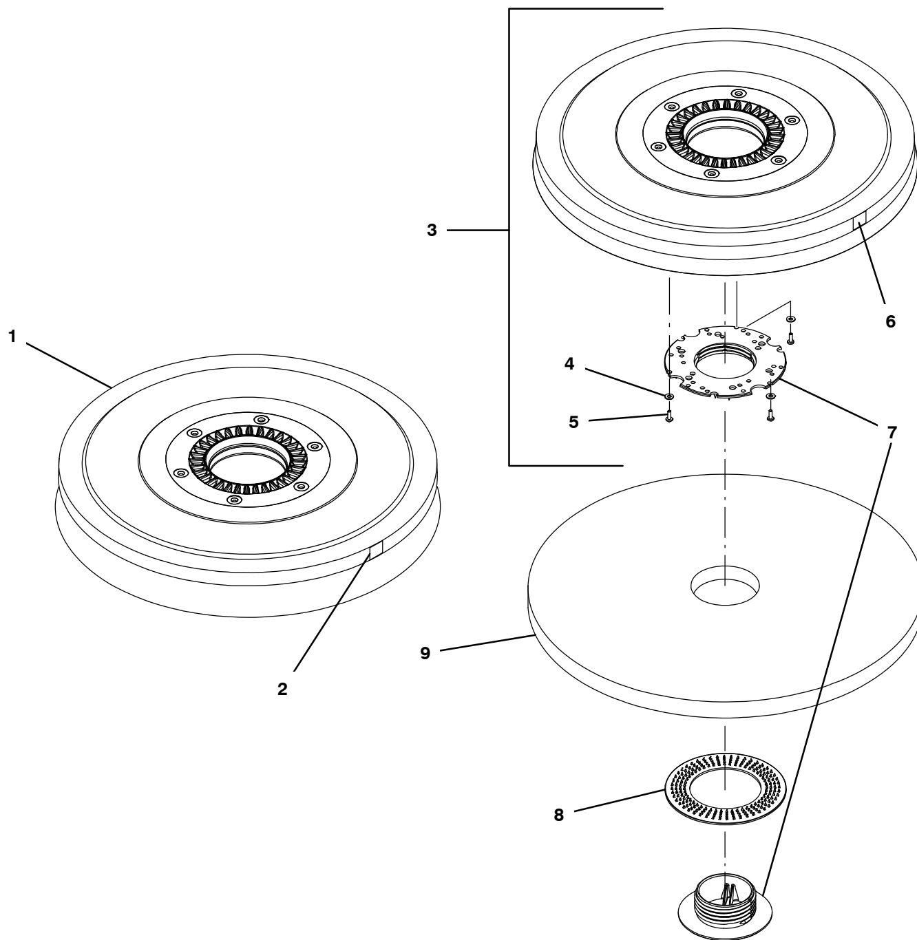
Fig. 2 – Brushes and Pad Driver Group, 500MM Disk Magnetic Hub
